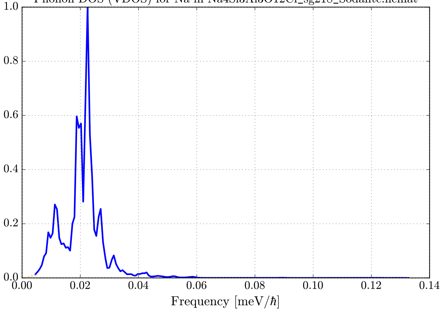
Phonon DOS (VDOS) for Na in Na 4 Si 3 Al 3 O 12 Cl_sg218_Sodalite.ncmat
