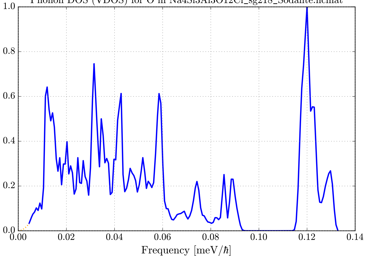
Phonon DOS (VDOS) for O in Na 4 Si 3 Al 3 O 12 Cl_sg218_Sodalite.ncmat
