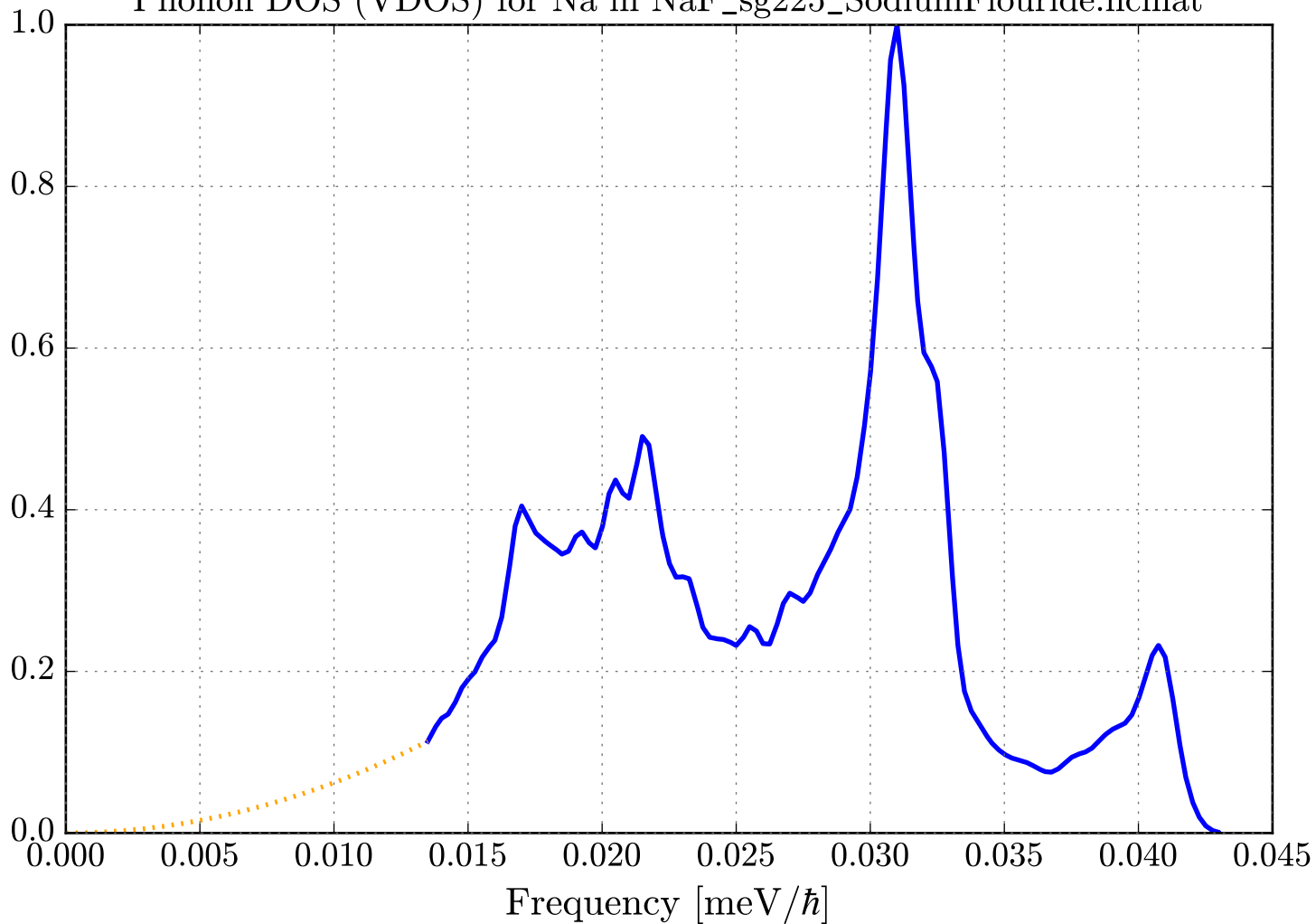
Phonon DOS (VDOS) for Na in NaF_sg225_SodiumFlouride.ncmat
