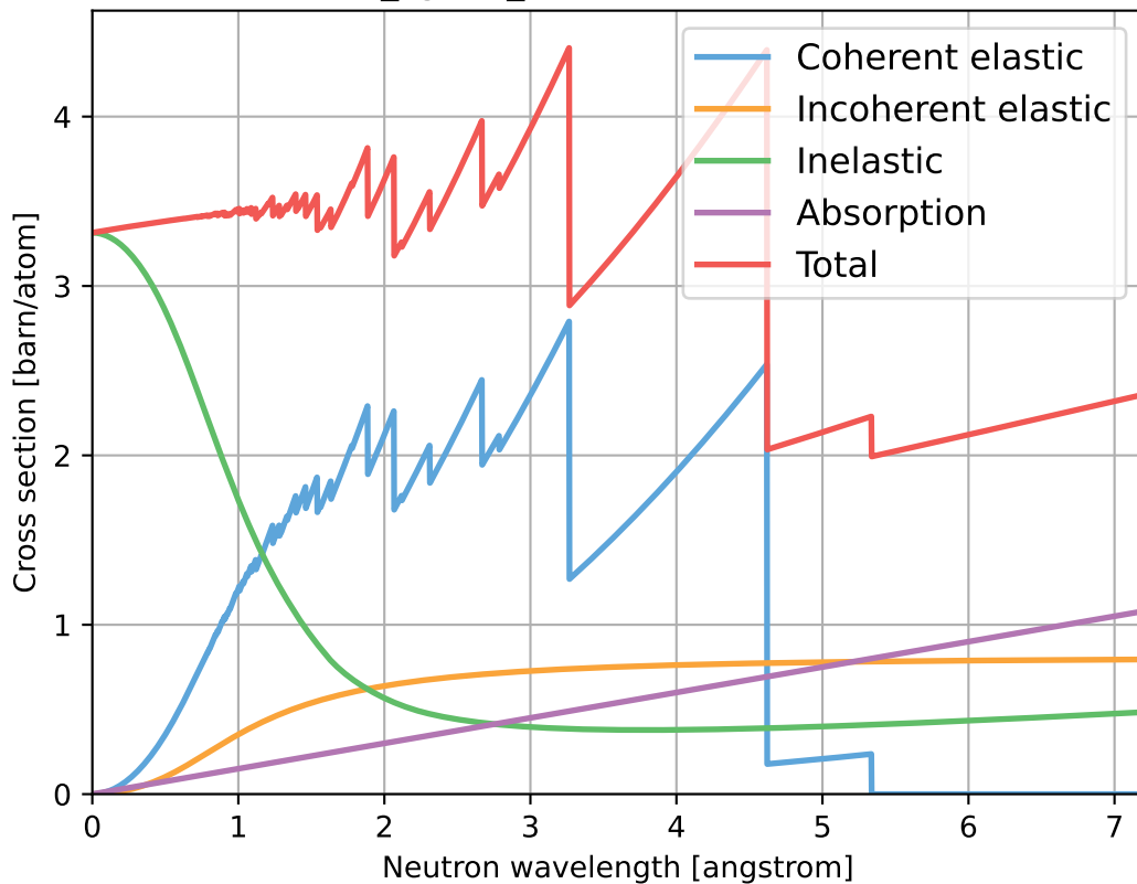
NaF_sg225_SodiumFlouride.ncmat
