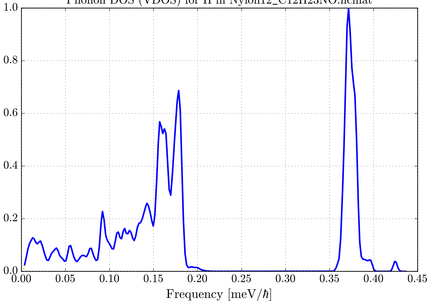
Phonon DOS (VDOS) for H in Nylon12_C12H23NO.ncmat
