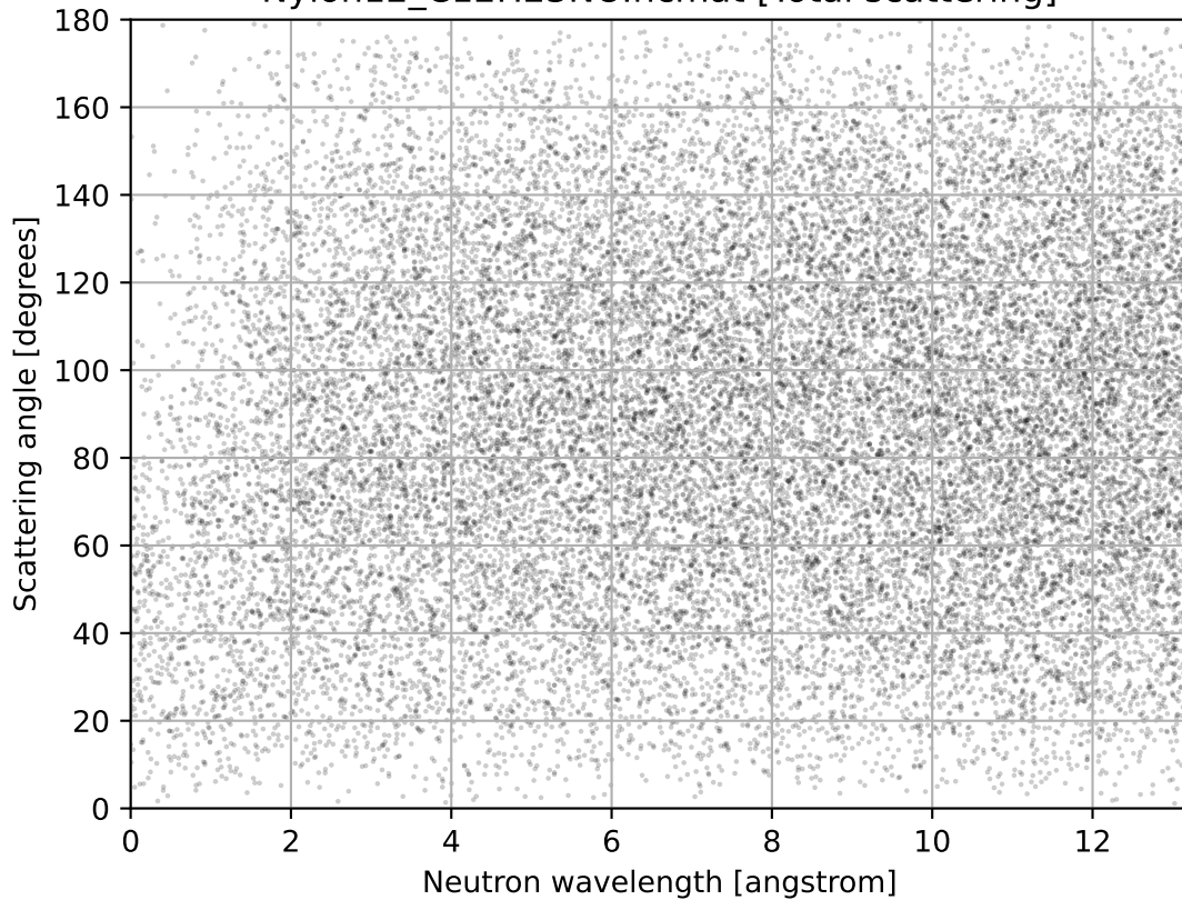
Nylon12_C12H23NO.ncmat [Total scattering]
