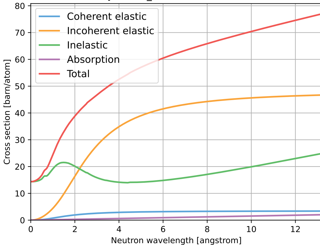
Nylon610_C16H30N2O2.ncmat
