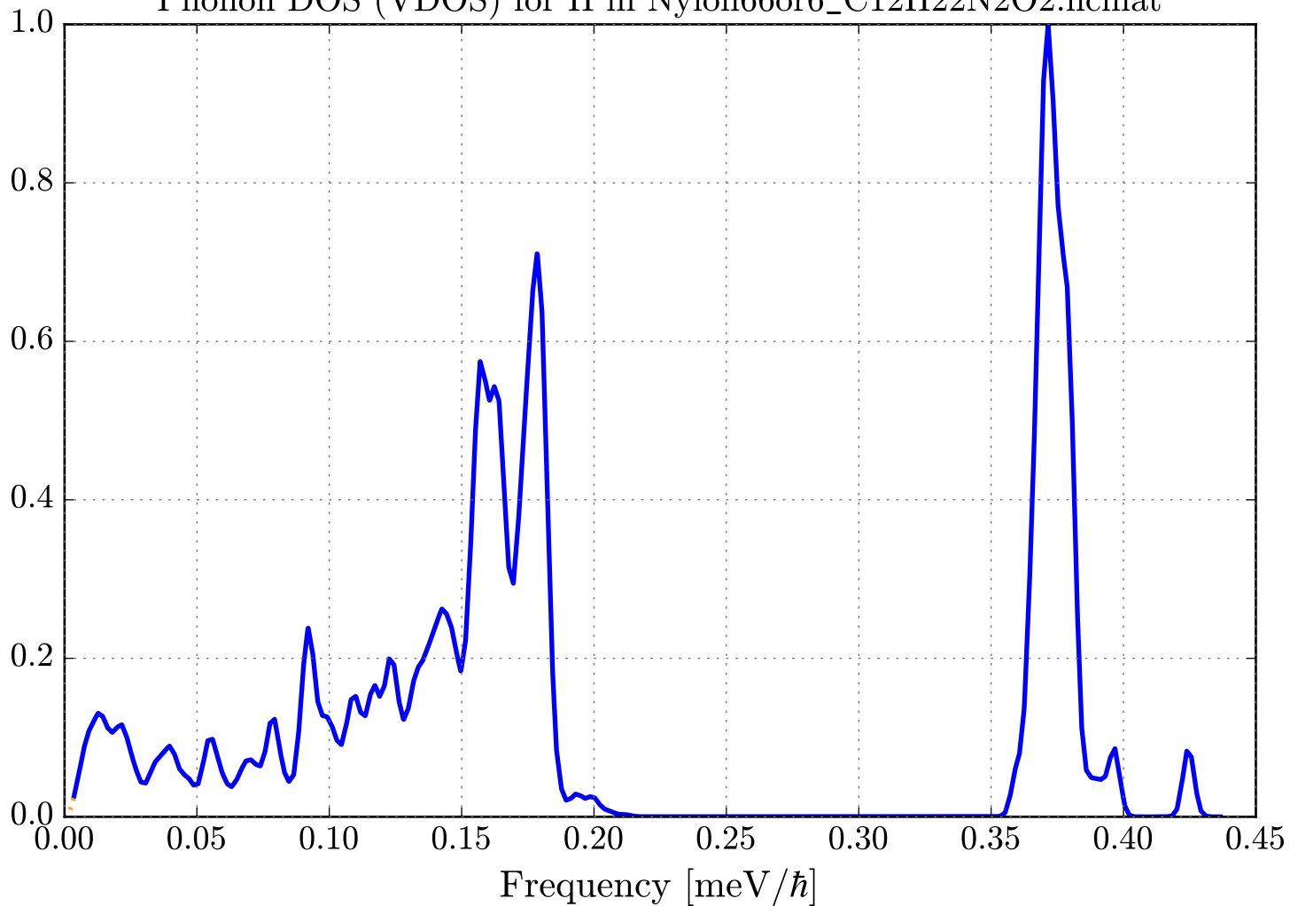
Phonon DOS (VDOS) for H in Nylon66or6_C12H22N2O2.ncmat
