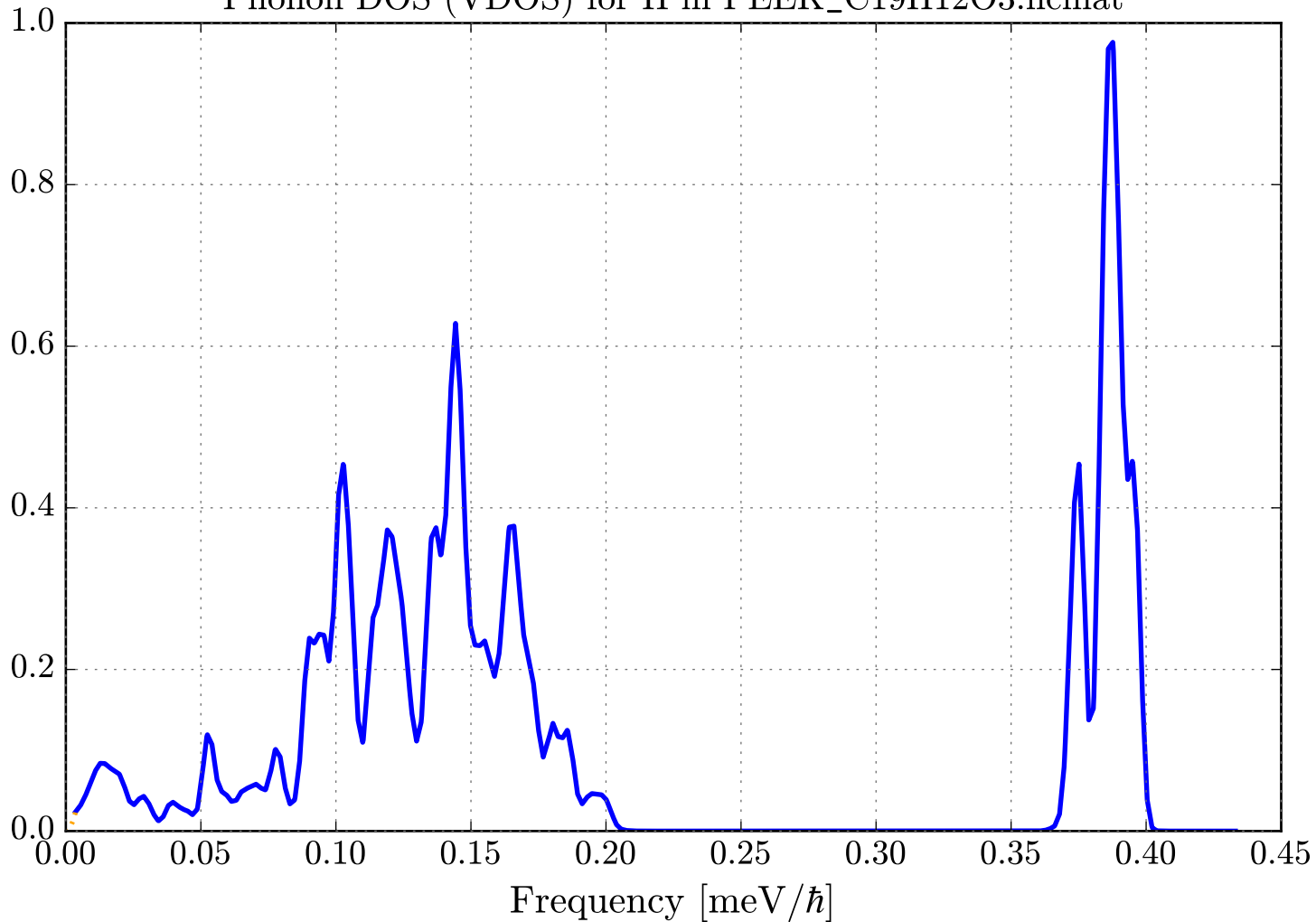
Phonon DOS (VDOS) for H in PEEK_C19H12O3.ncmat
