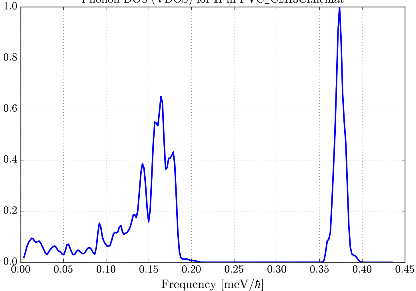
Phonon DOS (VDOS) for H in PVC_C2H3Cl.ncmat
