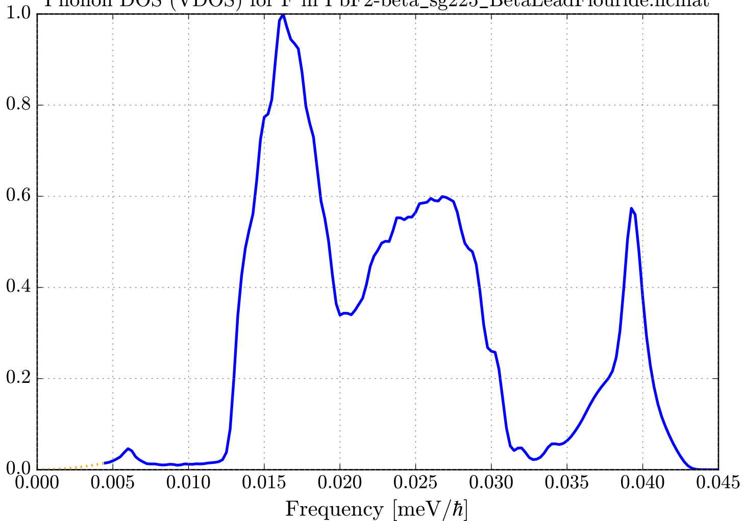
Phonon DOS (VDOS) for F in PbF2-beta_sg225_BetaLeadFlouride.ncmat
