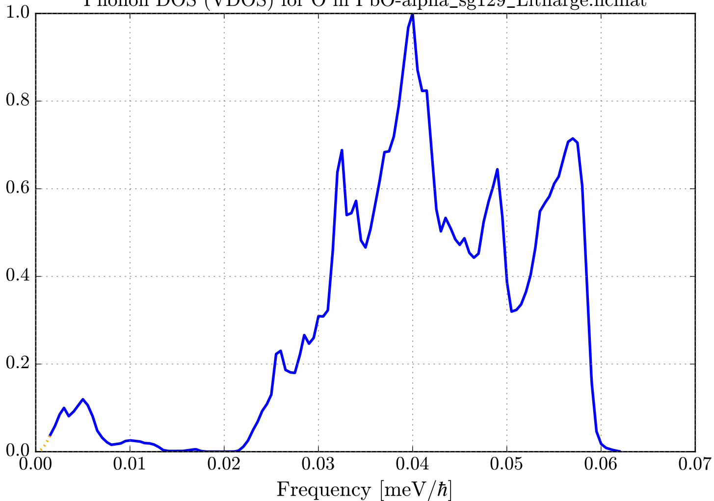
Phonon DOS (VDOS) for O in PbO-alpha_sg129_Litharge.ncmat
