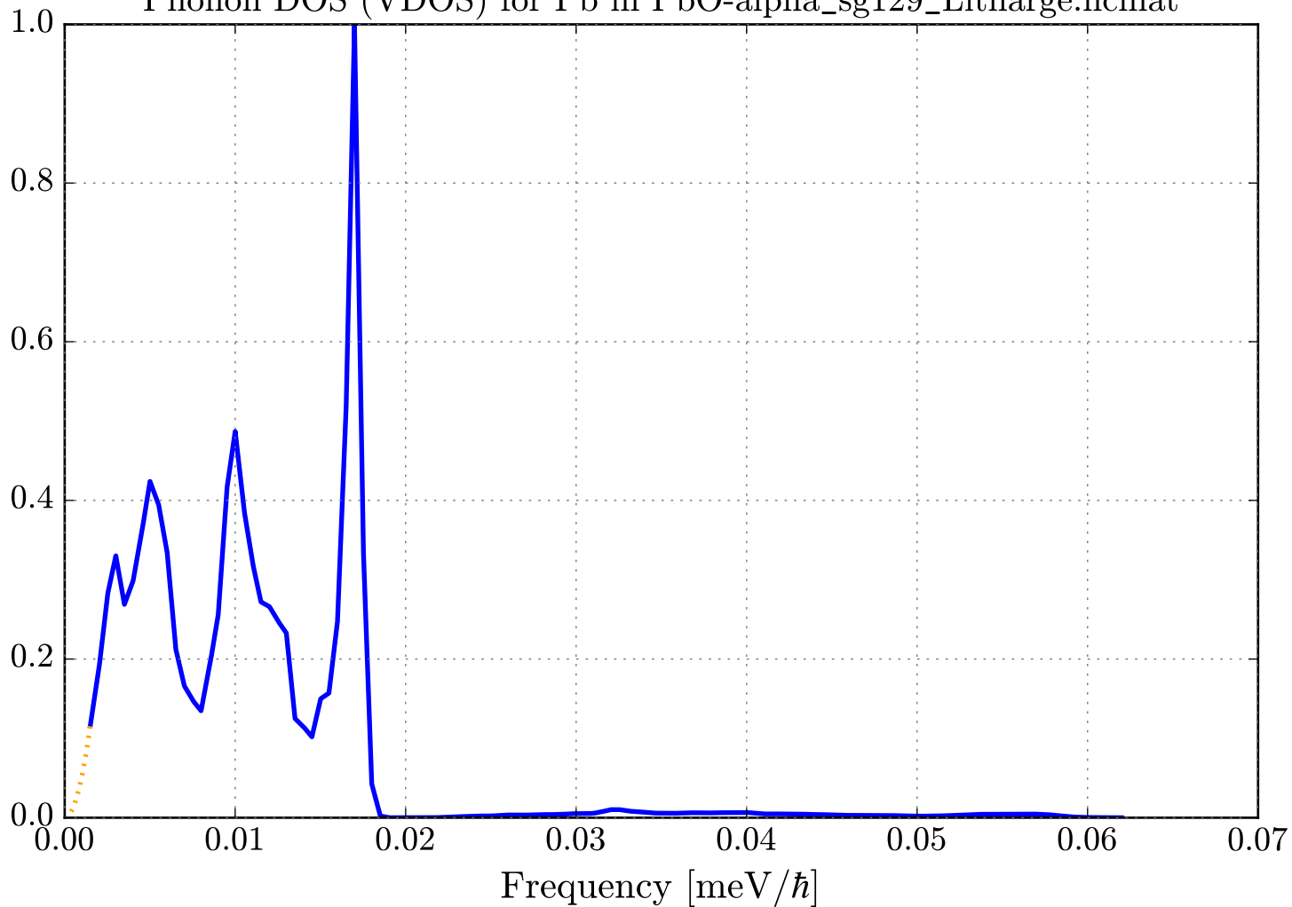
Phonon DOS (VDOS) for Pb in PbO-alpha_sg129_Litharge.ncmat
