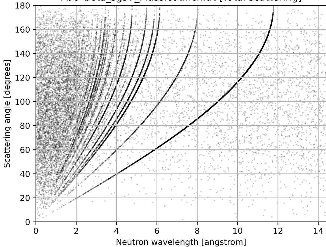
PbO-beta_sg57_Massicot.ncmat [Total scattering]
