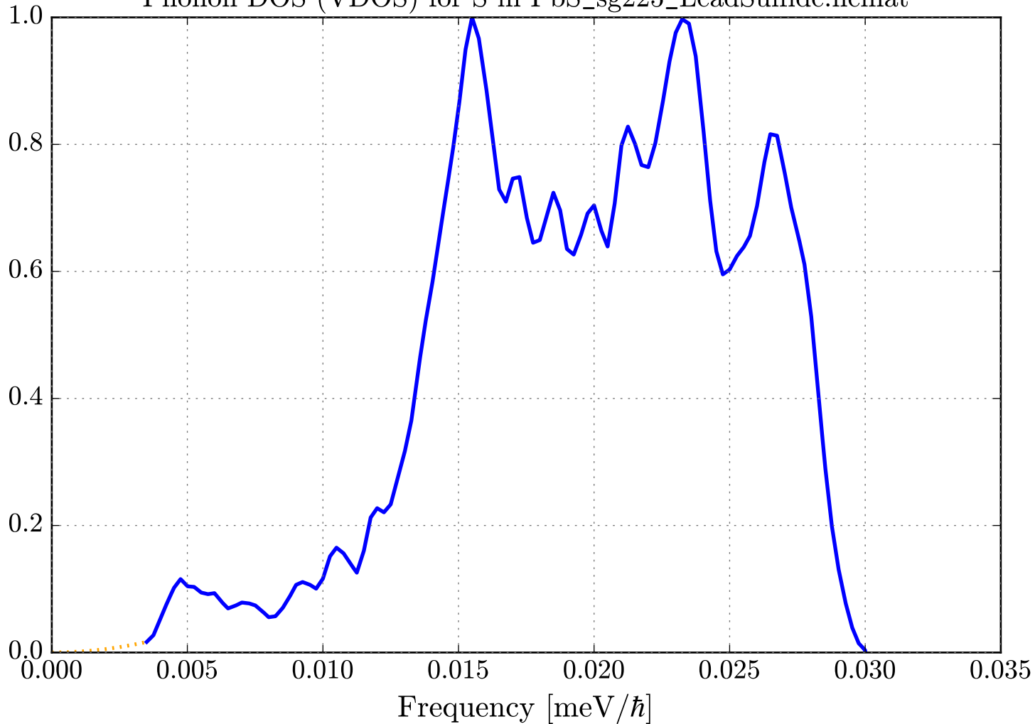
Phonon DOS (VDOS) for S in PbS_sg225_LeadSulfide.ncmat
