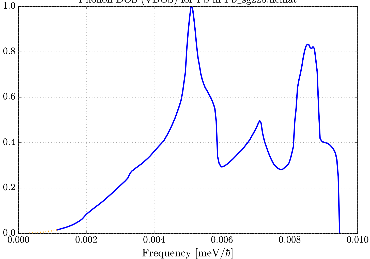
Phonon DOS (VDOS) for Pb in Pb_sg225.ncmat
