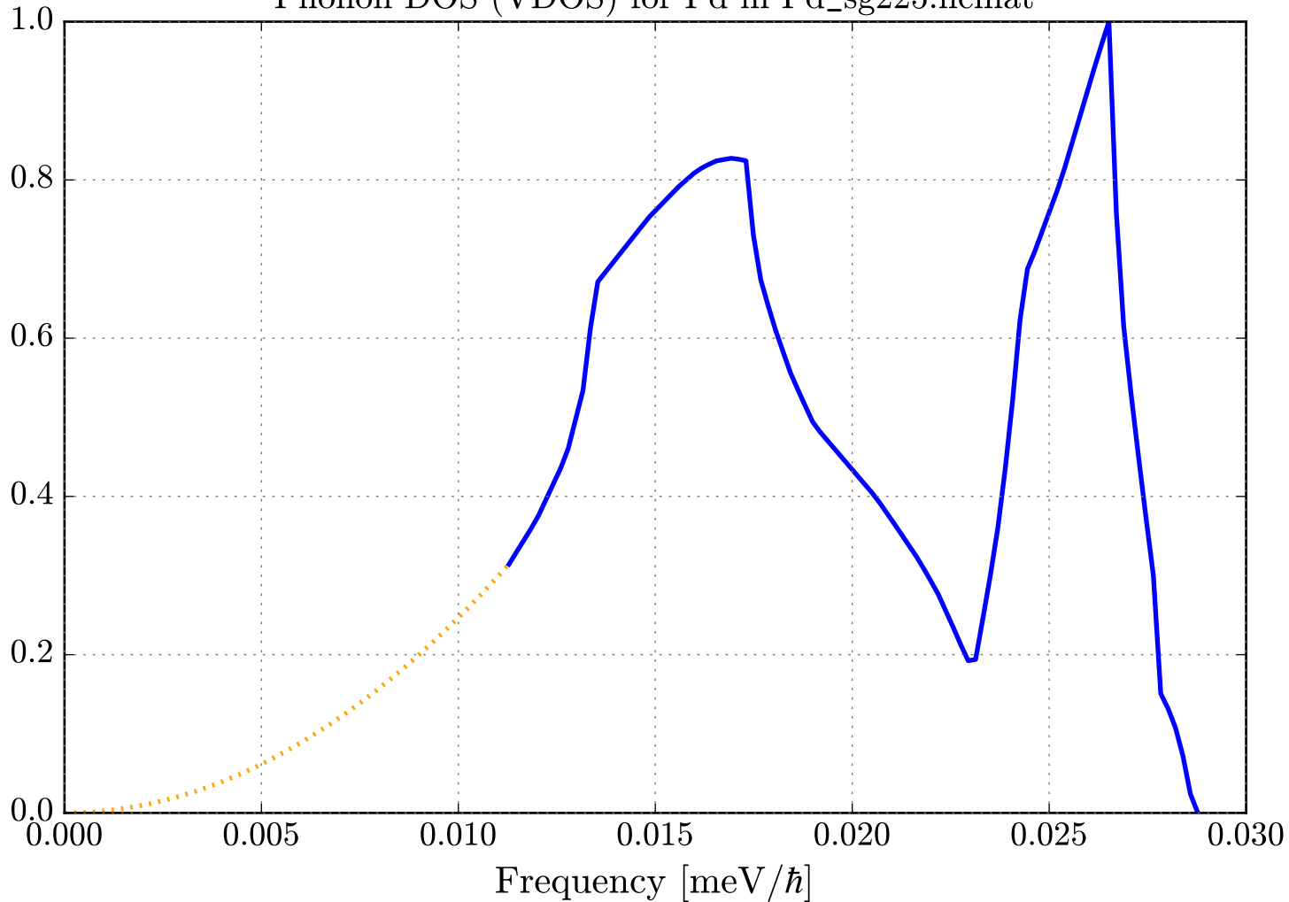
Phonon DOS (VDOS) for Pd in Pd_sg225.ncmat
