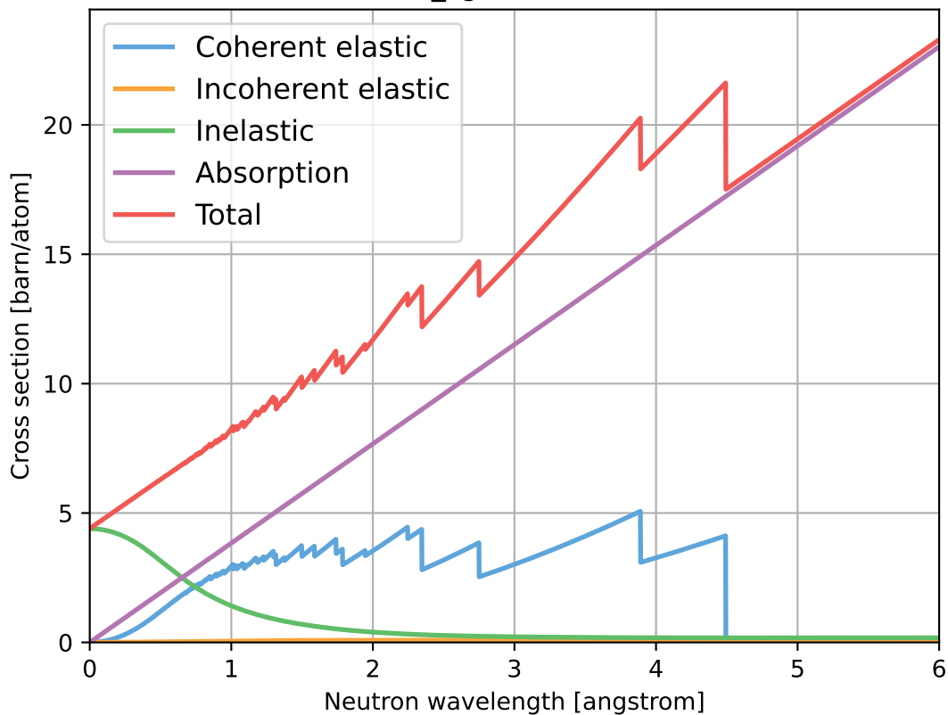
Pd_sg225.ncmat
