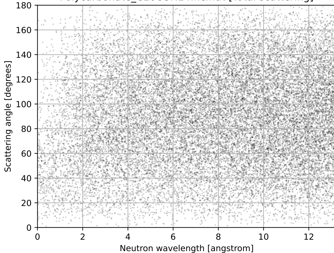
Polycarbonate_C16O3H14.ncmat [Total scattering]
