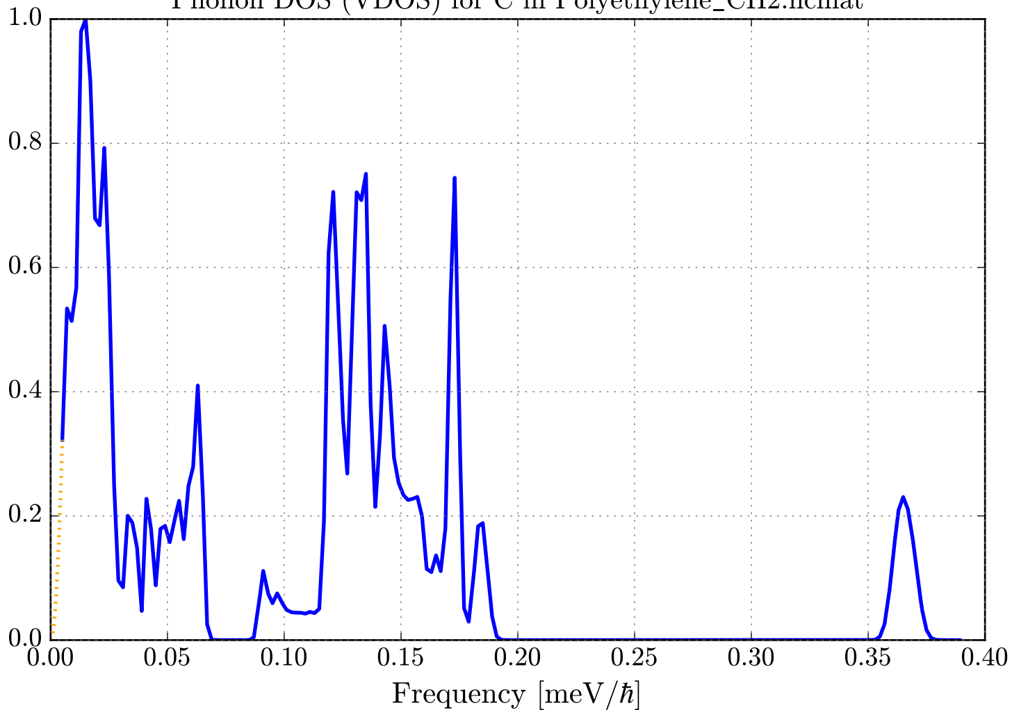
Phonon DOS (VDOS) for C in Polyethylene_CH2.ncmat
