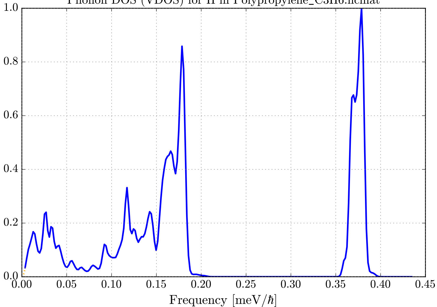
Phonon DOS (VDOS) for H in Polypropylene_C3H6.ncmat
