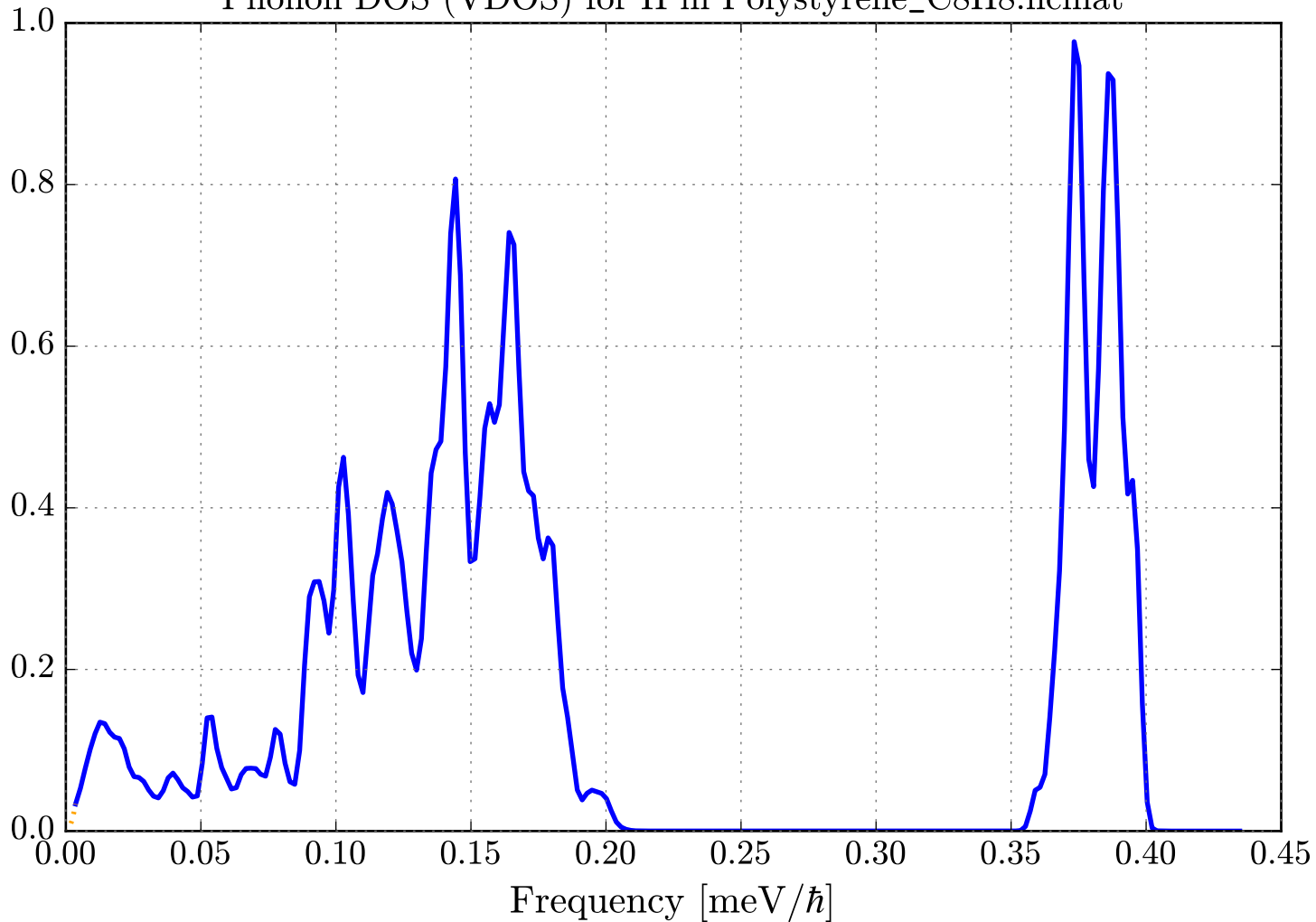
Phonon DOS (VDOS) for H in Polystyrene_C8H8.ncmat
