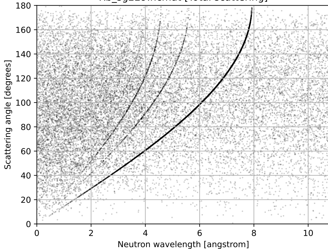
Rb_sg229.ncmat [Total scattering]
