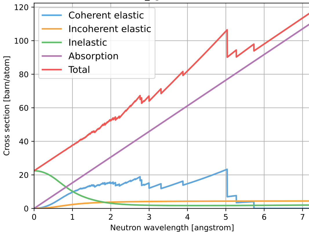
Sc_sg194.ncmat
