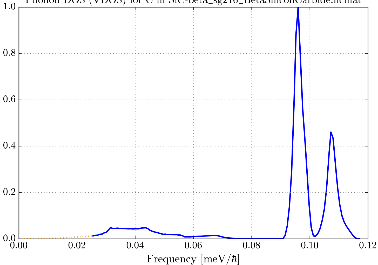
Phonon DOS (VDOS) for C in SiC-beta_sg216_BetaSiliconCarbide.ncmat
