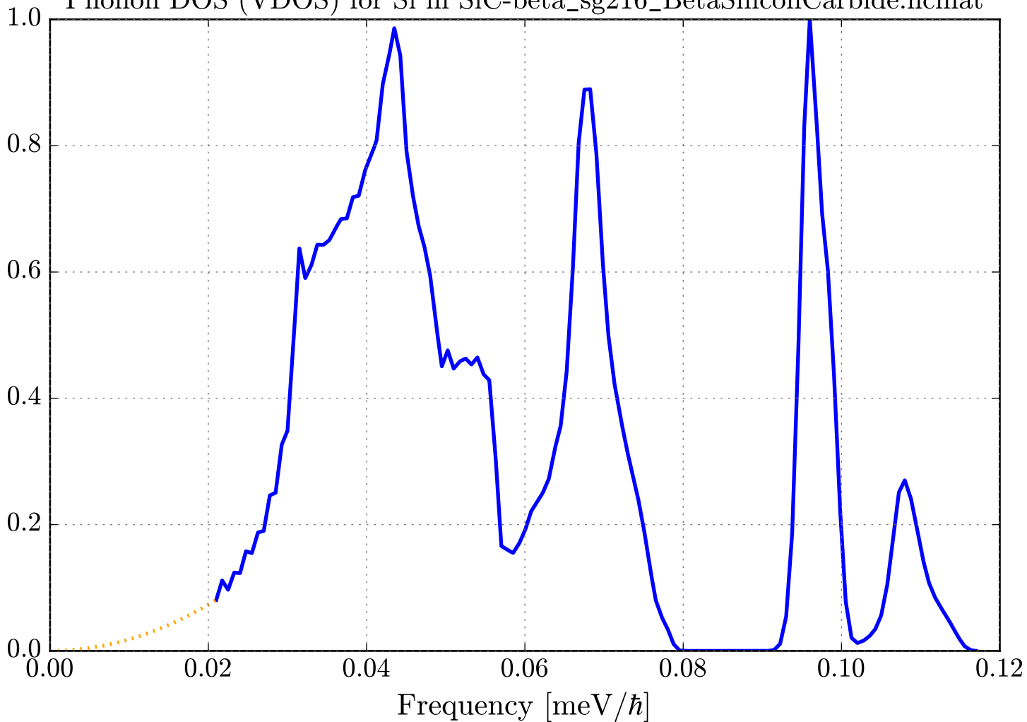
Phonon DOS (VDOS) for Si in SiC-beta_sg216_BetaSiliconCarbide.ncmat
