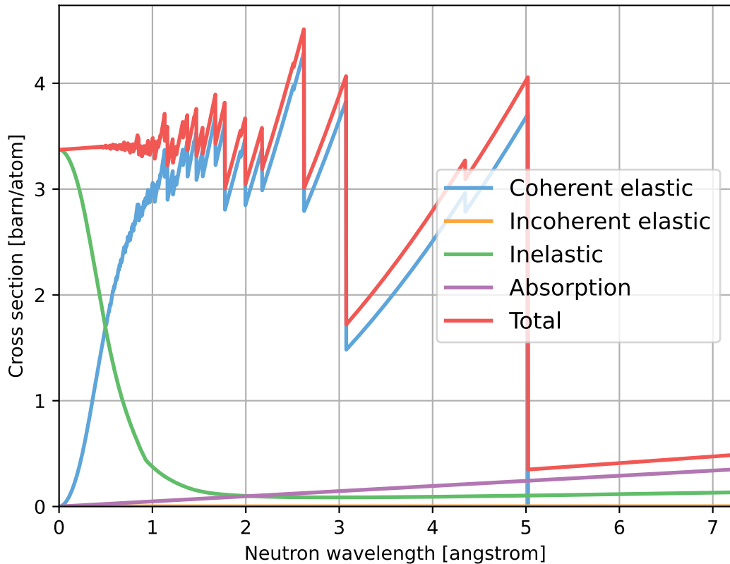
SiC-beta_sg216_BetaSiliconCarbide.ncmat
