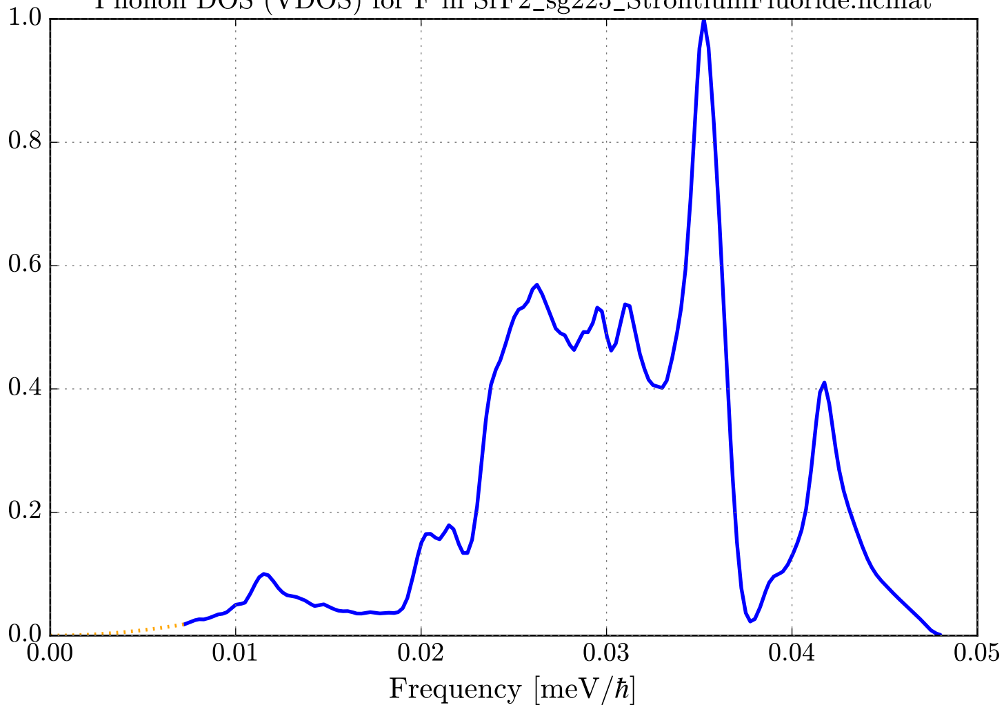
Phonon DOS (VDOS) for F in SrF2_sg225_StrontiumFluoride.ncmat
