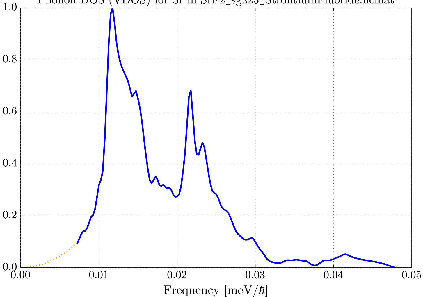
Phonon DOS (VDOS) for Sr in SrF2_sg225_StrontiumFluoride.ncmat
