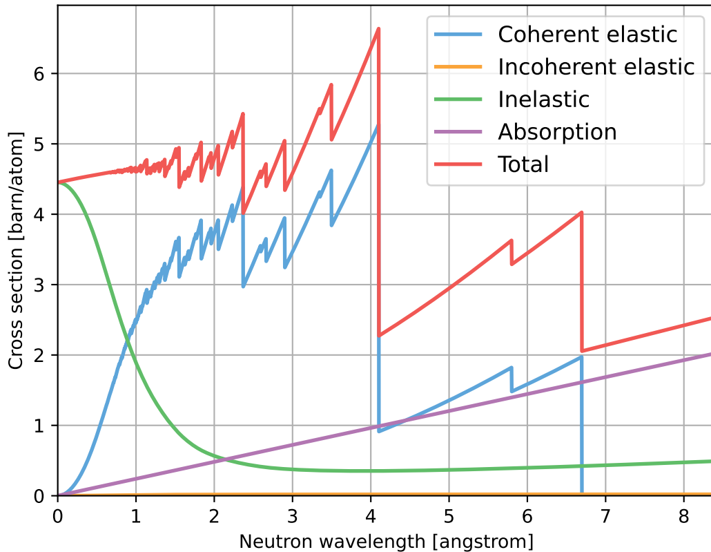
SrF2_sg225_StrontiumFluoride.ncmat
