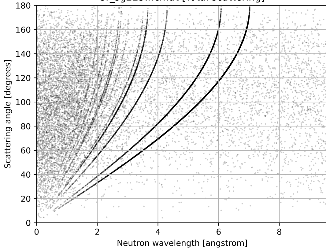
Sr_sg225.ncmat [Total scattering]
