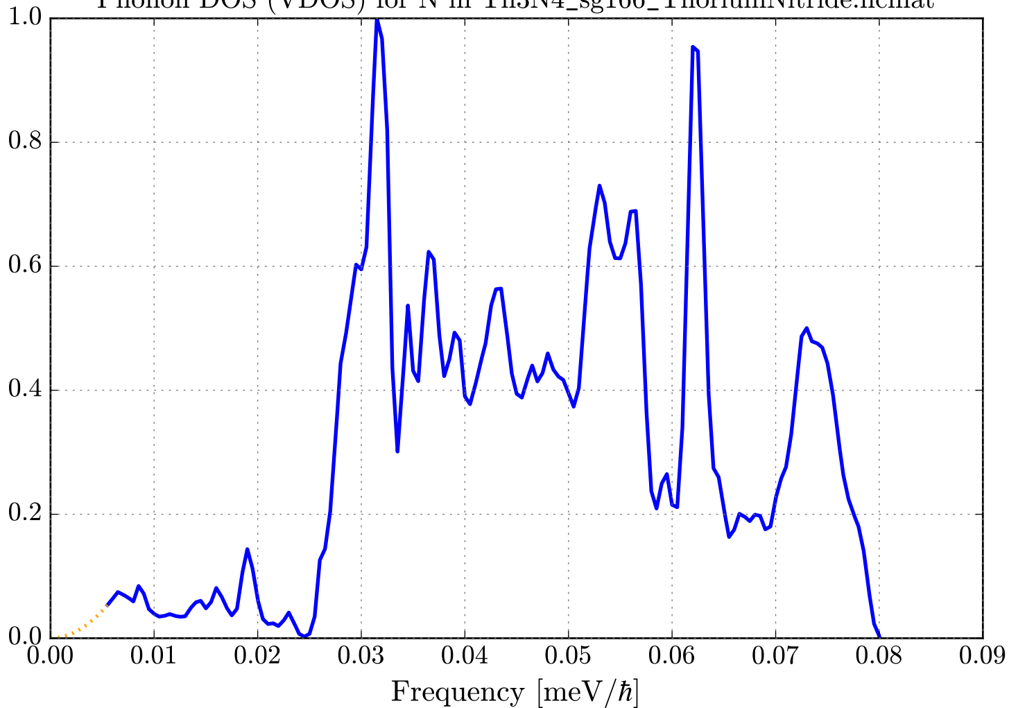
Phonon DOS (VDOS) for N in Th3N4_sg166_ThoriumNitride.ncmat
