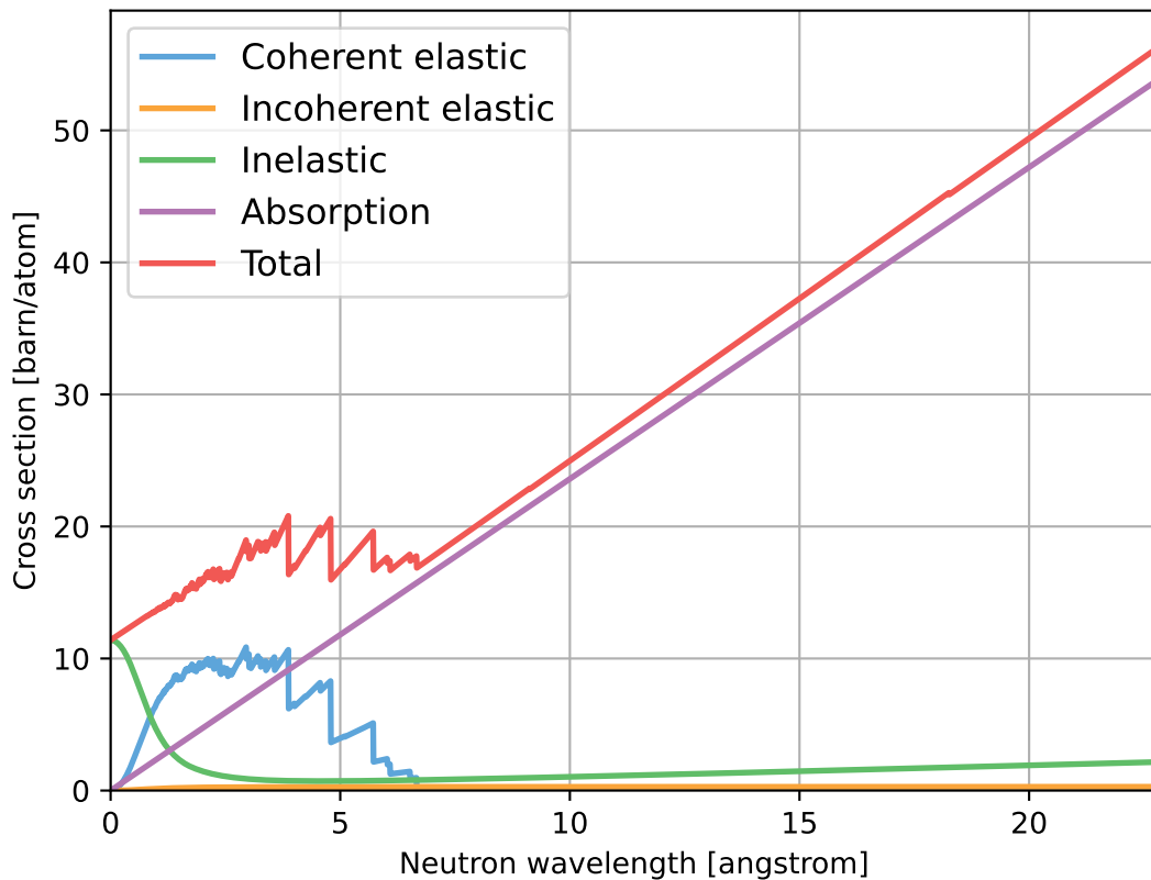
Th3N4_sg166_ThoriumNitride.ncmat
