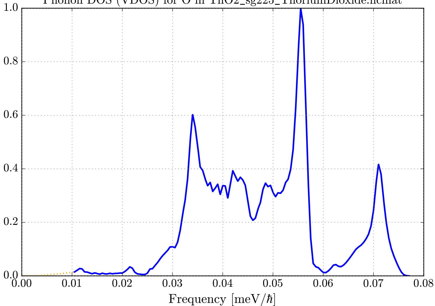
Phonon DOS (VDOS) for O in ThO2_sg225_ThoriumDioxide.ncmat
