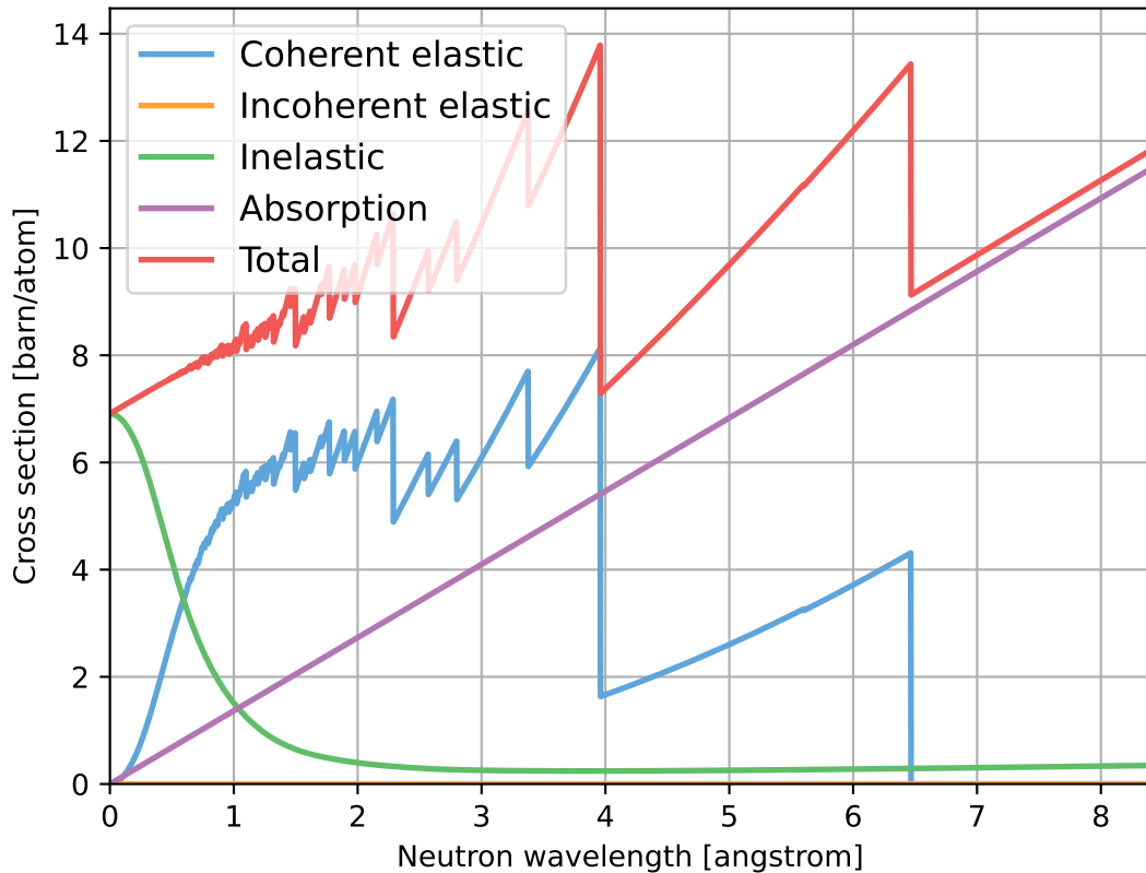
ThO2_sg225_ThoriumDioxide.ncmat
