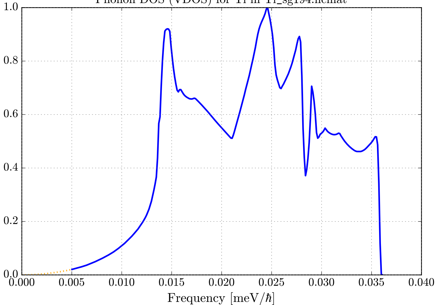
Phonon DOS (VDOS) for Ti in Ti_sg194.ncmat
