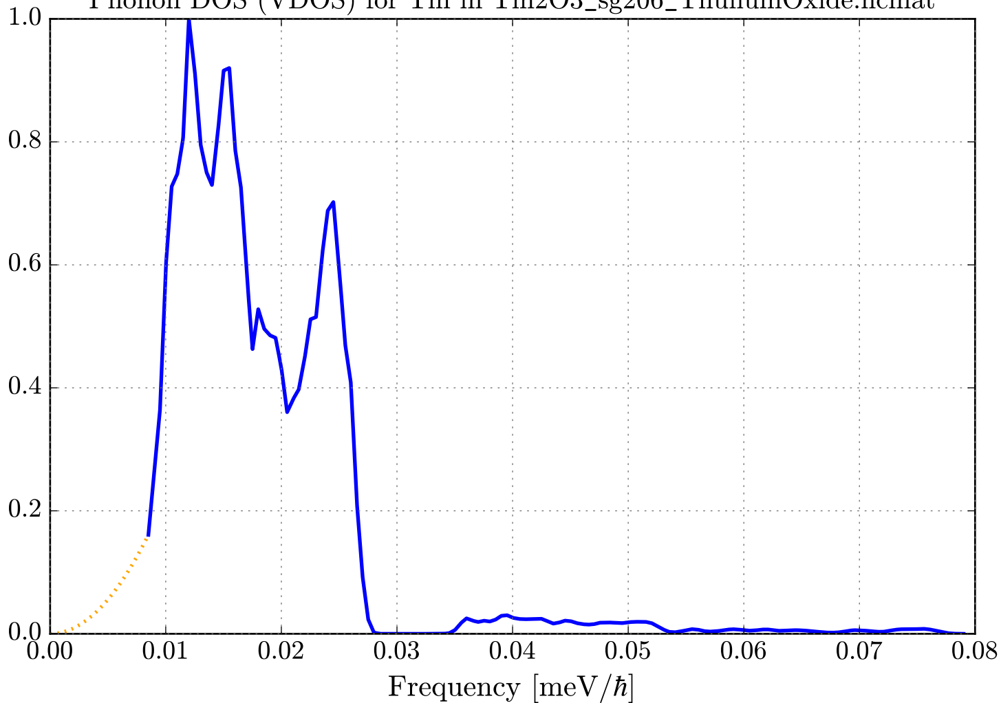
Phonon DOS (VDOS) for Tm in Tm2O3_sg206_ThuliumOxide.ncmat
