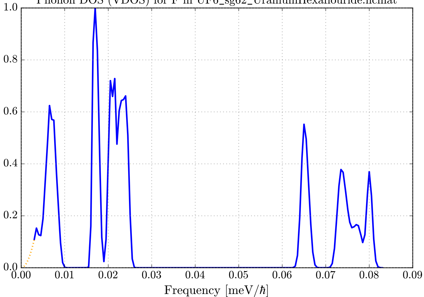
Phonon DOS (VDOS) for F in UF6_sg62_UraniumHexafluoride.ncmat
