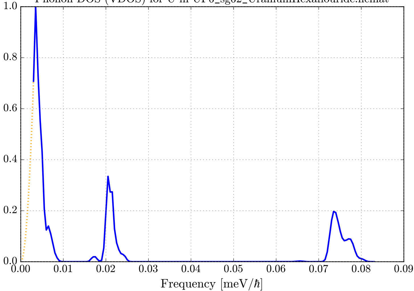
Phonon DOS (VDOS) for U in UF6_sg62_UraniumHexaflouride.ncmat
