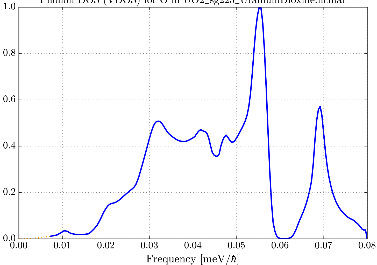
Phonon DOS (VDOS) for O in UO2_sg225_UraniumDioxide.ncmat
