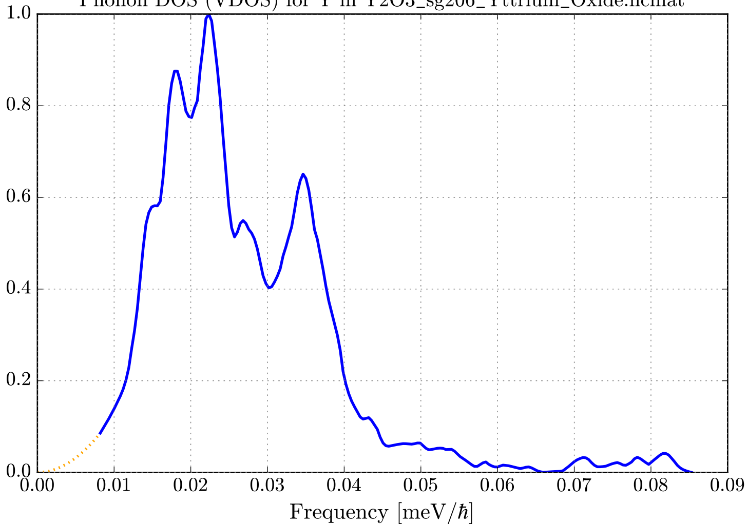
Phonon DOS (VDOS) for Y in Y2O3_sg206_Yttrium_Oxide.ncmat
