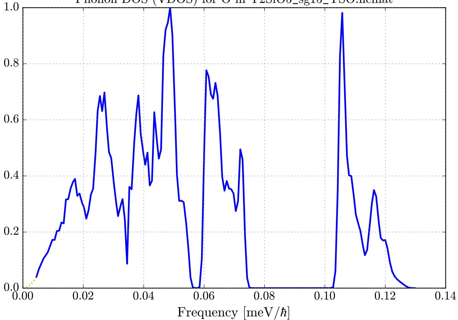
Phonon DOS (VDOS) for O in Y2SiO5_sg15_YSO.ncmat
