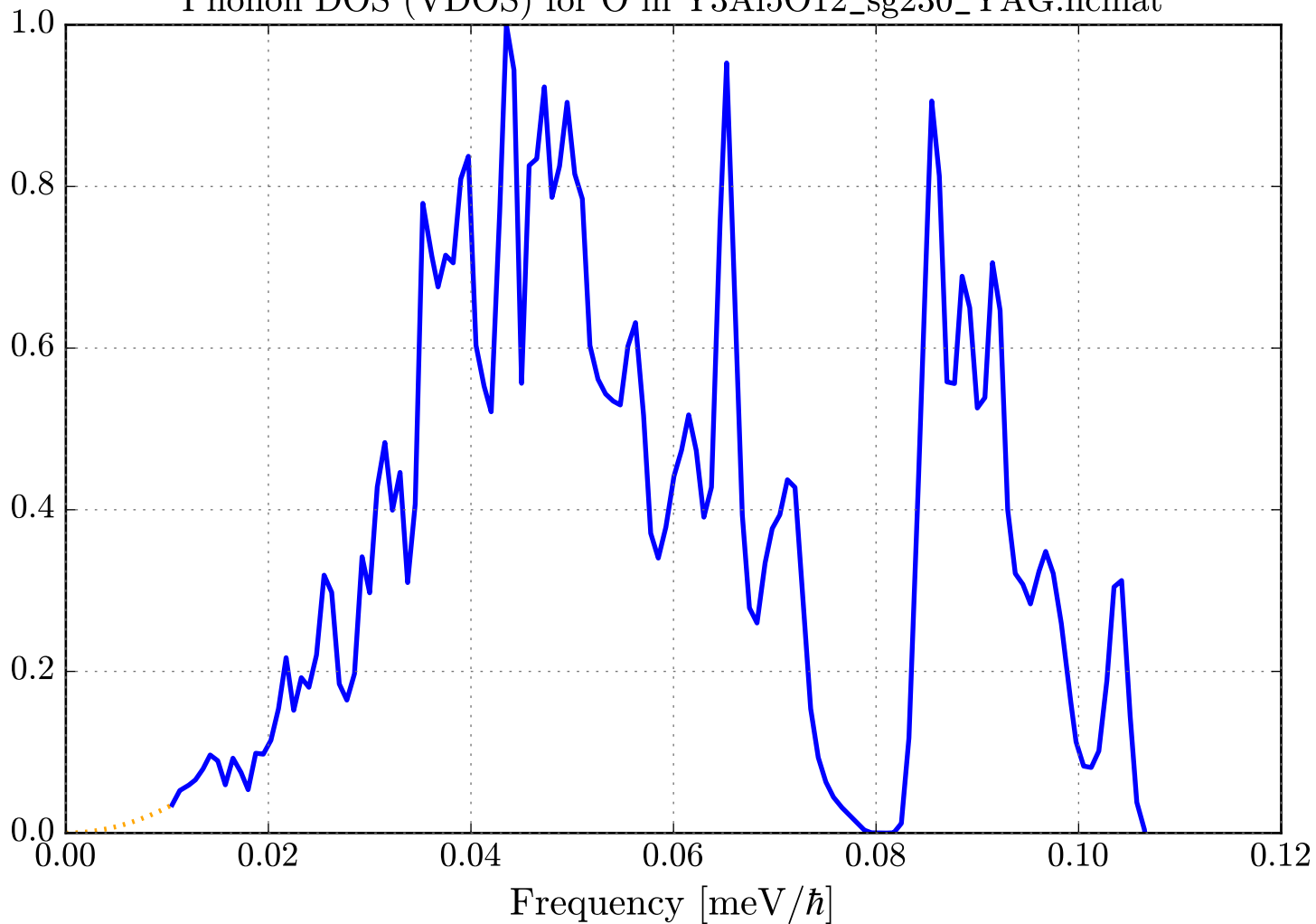
Phonon DOS (VDOS) for O in Y3Al5O12_sg230_YAG.ncmat
