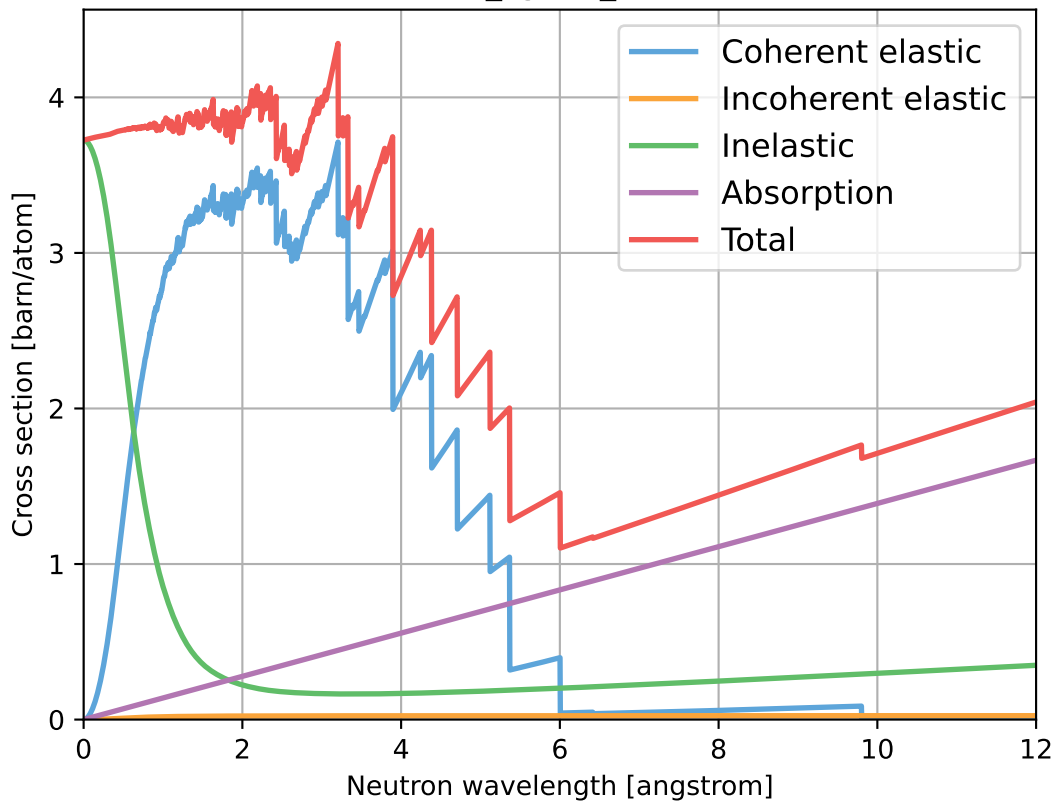
Y3Al5O12_sg230_YAG.ncmat
