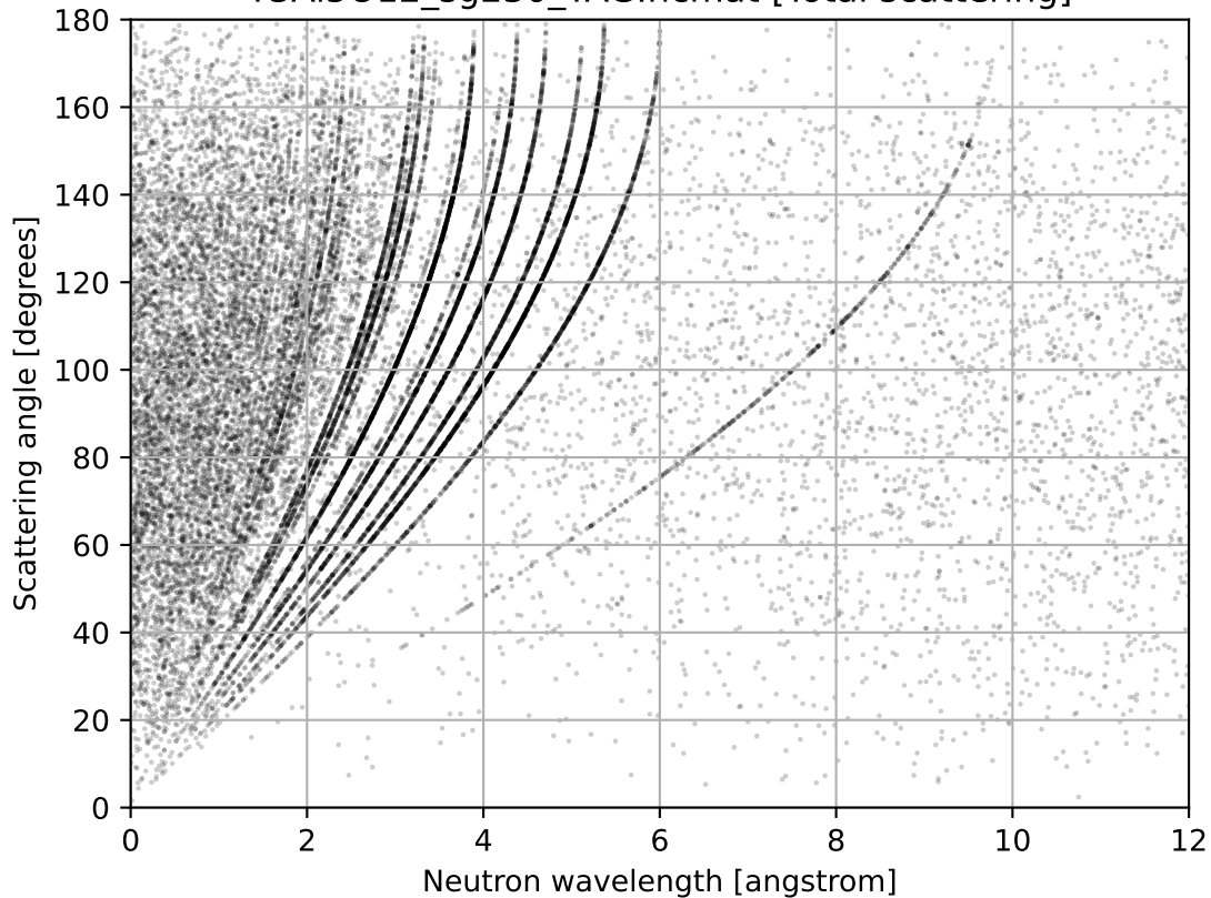
Y3A15O12_sg230_YAG.ncmat [Total scattering]
