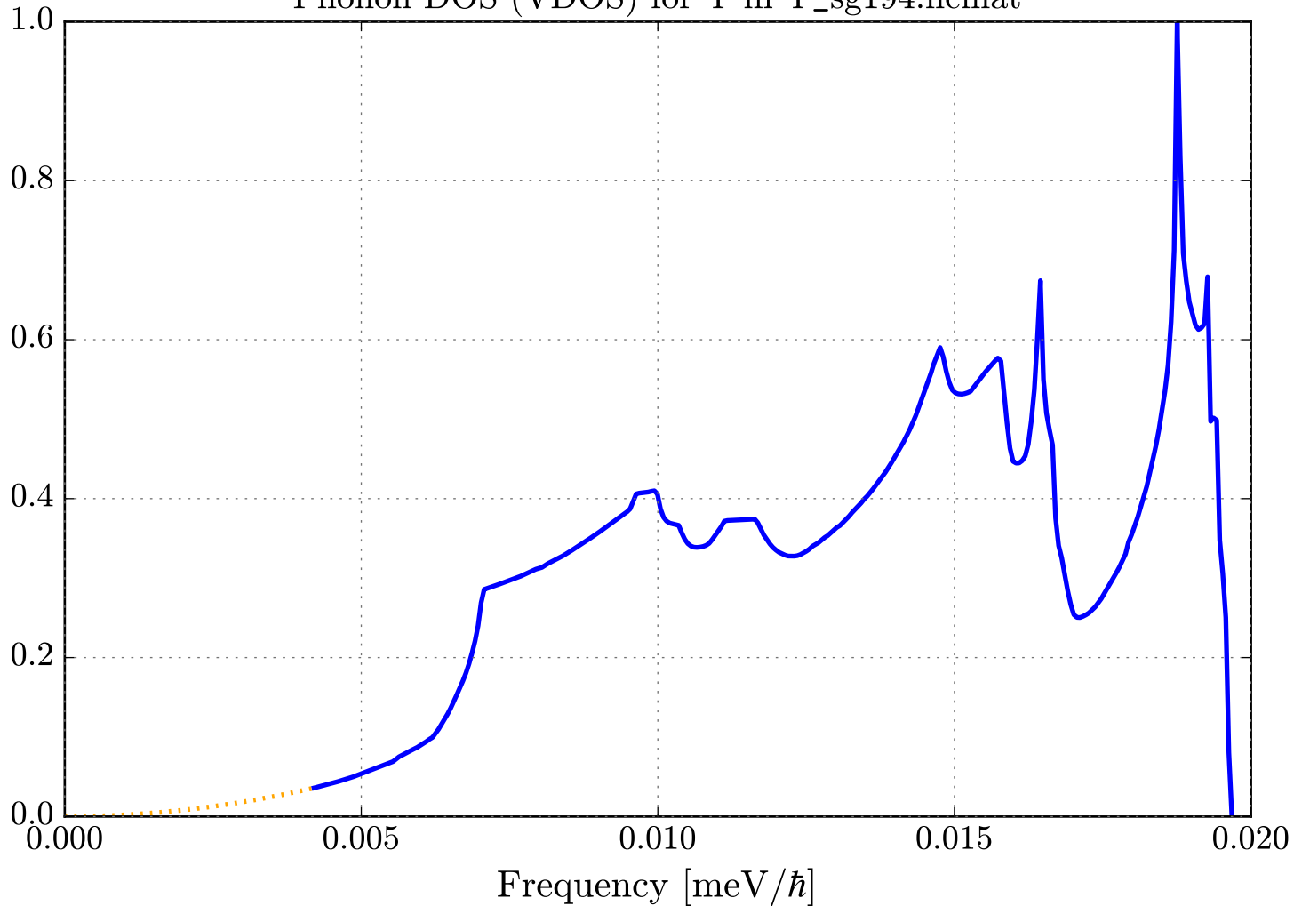
Phonon DOS (VDOS) for Y in Y_sg194.ncmat
