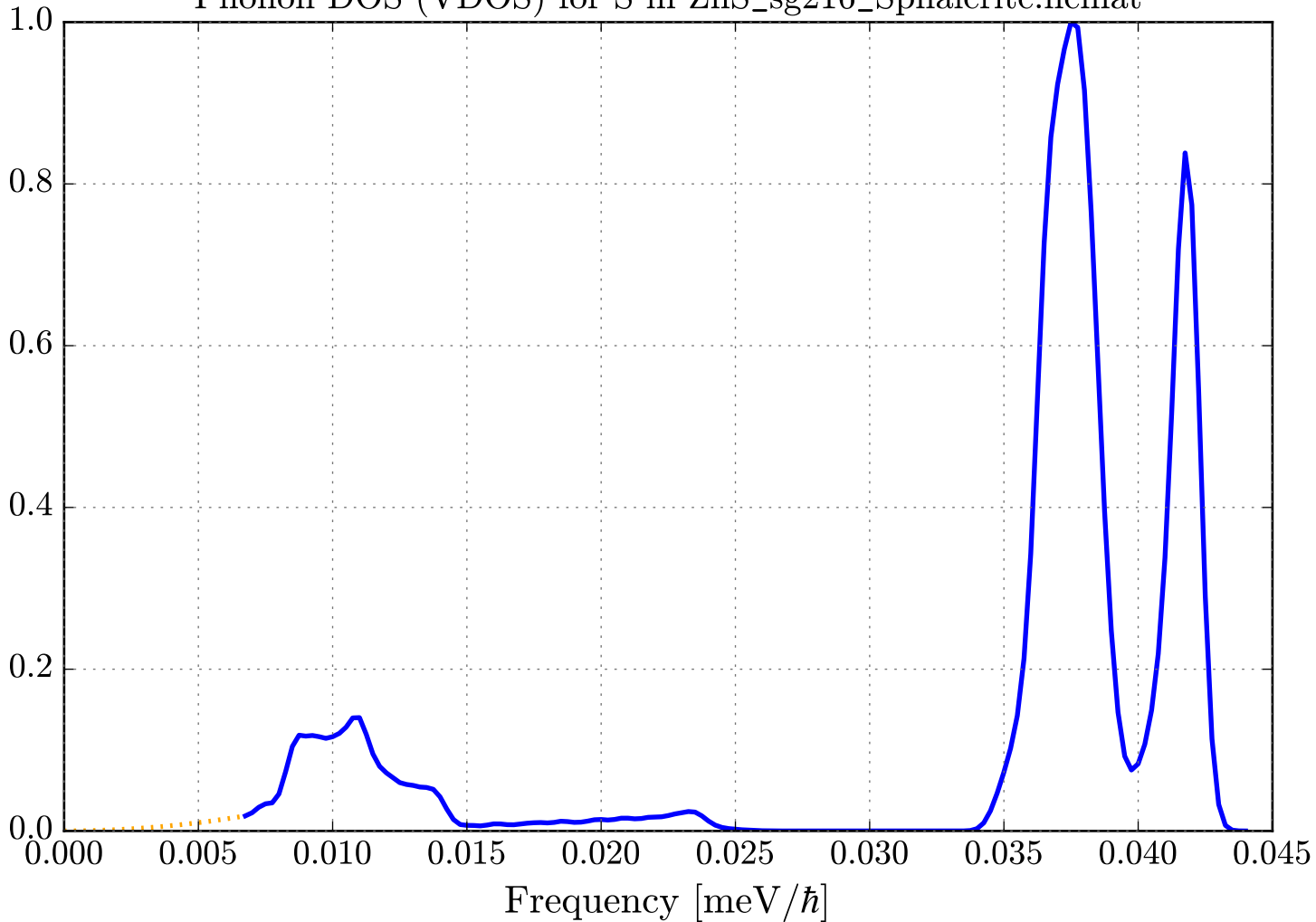
Phonon DOS (VDOS) for S in ZnS_sg216_Sphalerite.ncmat
