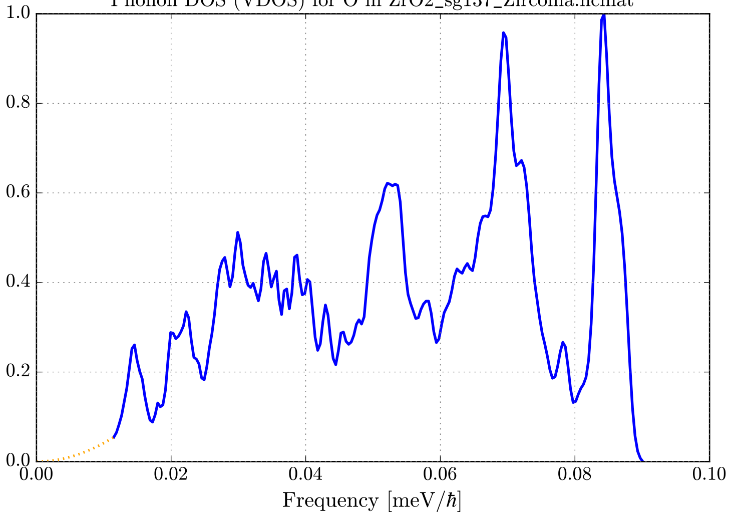
Phonon DOS (VDOS) for O in ZrO2_sg137_Zirconia.ncmat
