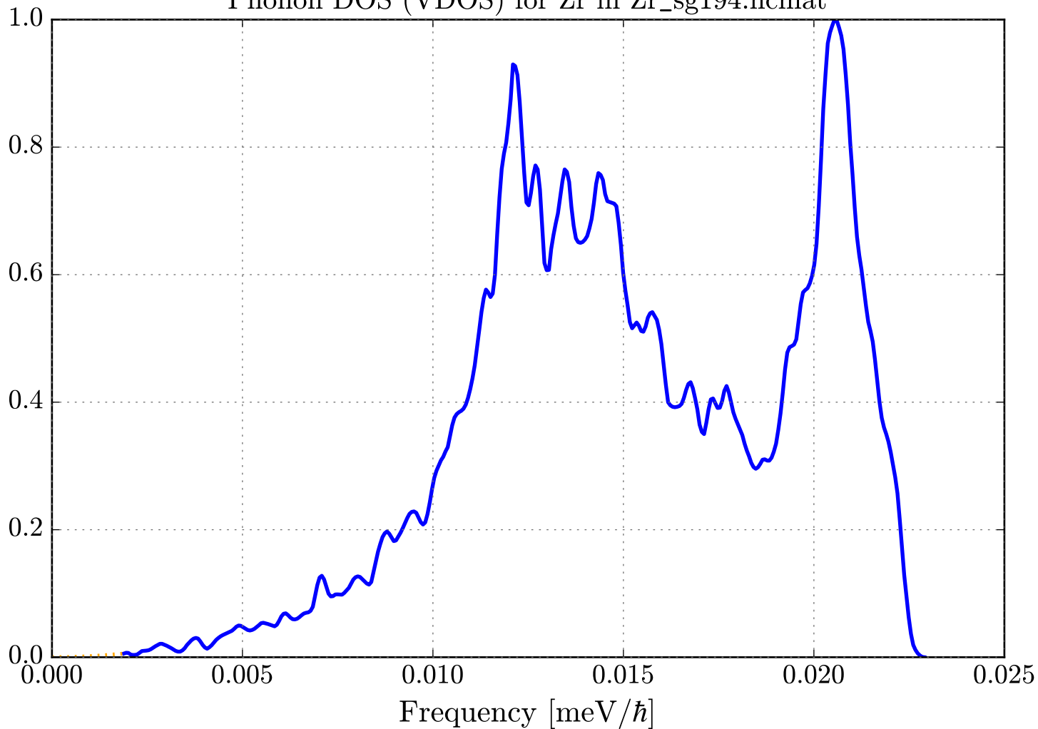
Phonon DOS (VDOS) for Zr in Zr_sg194.ncmat
