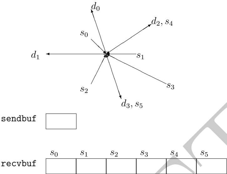
Figure 7.3: Neighborhood gather communication example.
