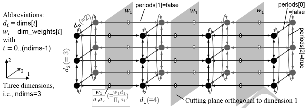
Figure 7.1: Example of a virtual process grid with 3 dimensions and 24 MPI processes. The arguments \text{dim\_weights}[i]_{i=0..(\text{ndims}-1)} , abbreviated with w_i , should be specified as the accumulated message size (in bytes) communicated in one communication step through each cutting plane orthogonal to dimension d_i and in each of the two directions. Based on the factorization of the number of processes into the d_i , the expected size of each message along the edges of the virtual process grid will be w_i / \prod_{j \neq i} d_j .
