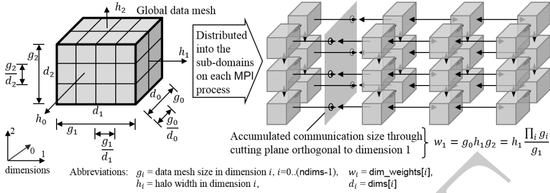
Figure 7.2: Example for the calculation of the accumulated communication size w_{i,i=0..2} in each dimension. The data mesh sizes g_{i,i=0..2} express the three dimensions of the total application data mesh. The value h_i represents the halo width in a given direction when the 2-dimensional side of a subdomain is communicated to the neighbor process in that direction. The values w_{i,i=0..2} are used as input argument dim_weights[i] in MPI_DIMS_CREATE_WEIGHTED or MPI_CART_CREATE_WEIGHTED , which return an optimized factorization of the number of processes into the dimensions of the virtual process grid, expressed by d_i . The figure shows the resulting division of the total application mesh into its subdomains.
