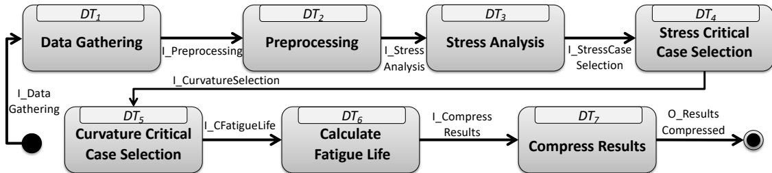
Figure 2.3: Risers Fatigue Analysis Workflow [48].
