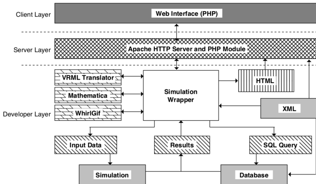
Figure 3.14: WBCSim approach architecture [82–84].
