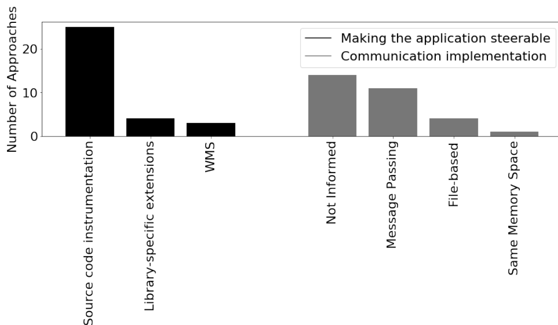
Figure 3.5: Summarization of Table 3.2.
