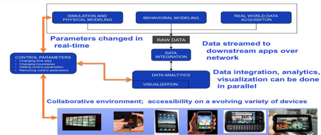
Figure 3.10: DANANI and D’AMORA [91]’ view on “the future of steering workflows”.
