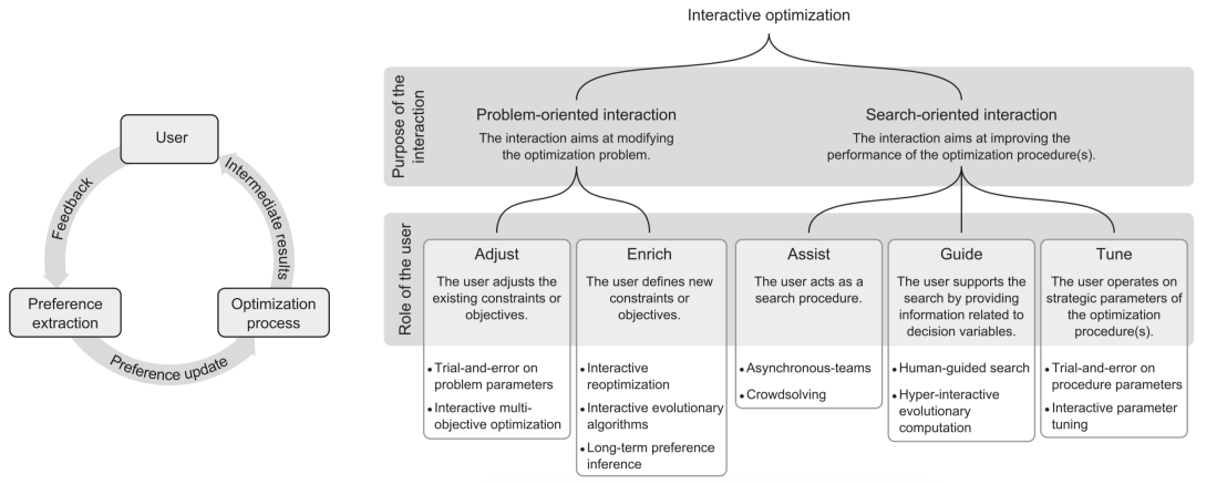
Figure 3.4: User steering approach for optimization [113].
