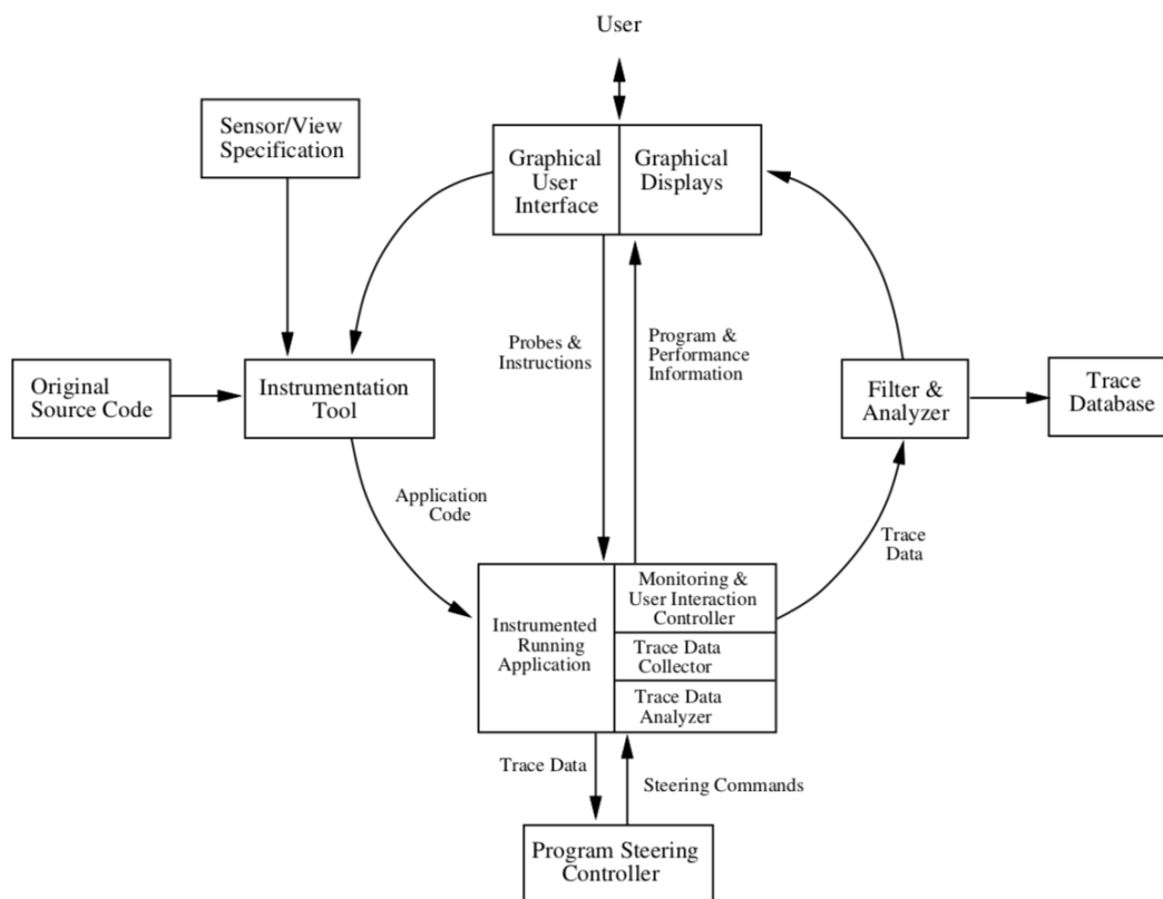
Figure 3.13: Falcon’s architecture [80].
