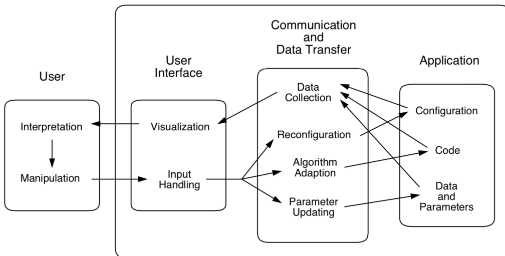
Figure 3.7: User steering concepts, according to MULDER et al. [54].
