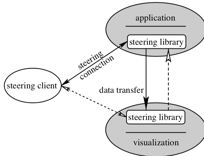
Figure 3.6: Basic components of an approach that supports user steering, according to PICKLES et al. [76].
