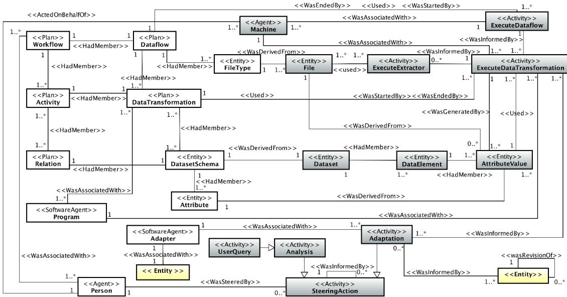
Figure 4.1: PROV-DfA overview. A larger visualization is on GitHub [126].
