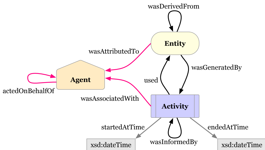
Figure 2.6: PROV-DM General Overview [50].
